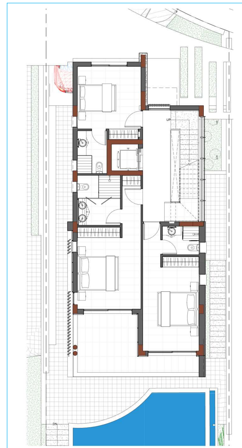
PRELIMINARY FIRST FLOOR PLAN
